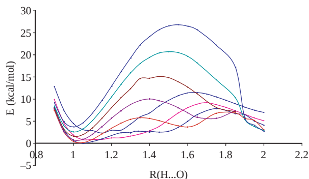
Figure 13. Proton transfer barriers as a function of R(H\cdots O) distance (in Å) in the methylethylammonium nitrate ionic liquid.
